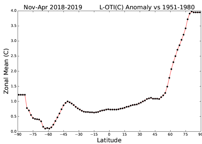
Figure 1. The temperature anomaly 90°S-90°N.
